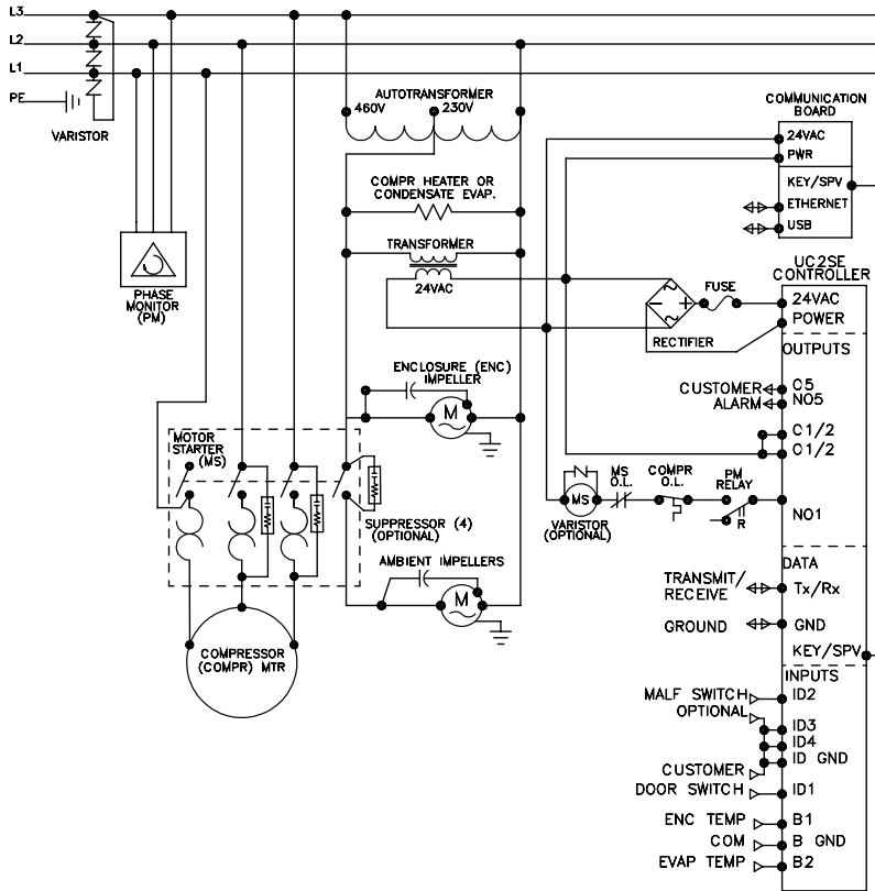
ELECTRICAL SCHEMATIC
