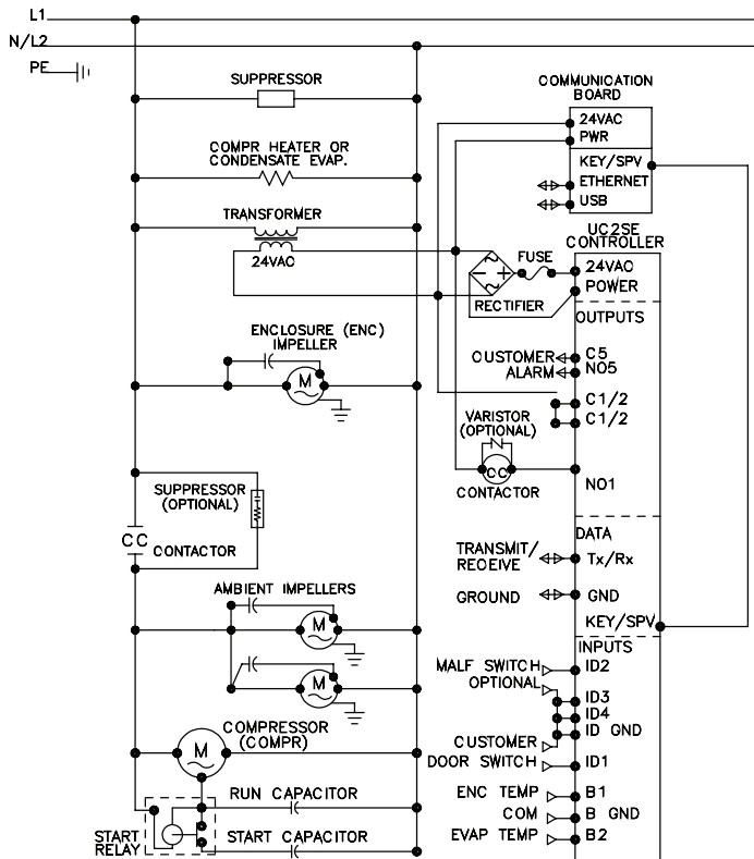
ELECTRICAL SCHEMATIC
